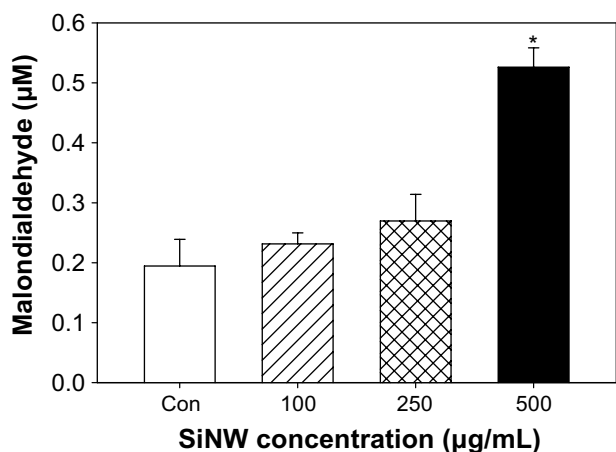
Figure 8. SiNW-induced lipid peroxidation. Exposure mixtures contained 5 \times 10^7 RAW 264.7 cells and 0, 100, 250, or 500 µg/mL SiNW. The data represent mean \pm SEM values of five independent experiments. *Different from the control ( P < 0.05 ).
