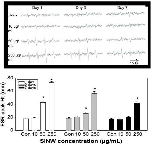
Figure 6. Reactivity ex vivo . ESR peak heights recorded after five minutes incubation at 37 °C, from a pH 7.4 phosphate buffered solution of 200 mM DMPO and the following reactants: pre-exposed rat AMs ( 10^6 /mL). The ESR spectrometer settings were: receiver gain, 2.5 \times 10^5 ; time constant, 0.25 seconds; modulation amplitude, 0.5 G; scan time, 8 minutes; magnetic field, 3375 \pm 100 G. The data represent mean \pm SEM values of four independent experiments. *Different from the control ( P < 0.05 ).
