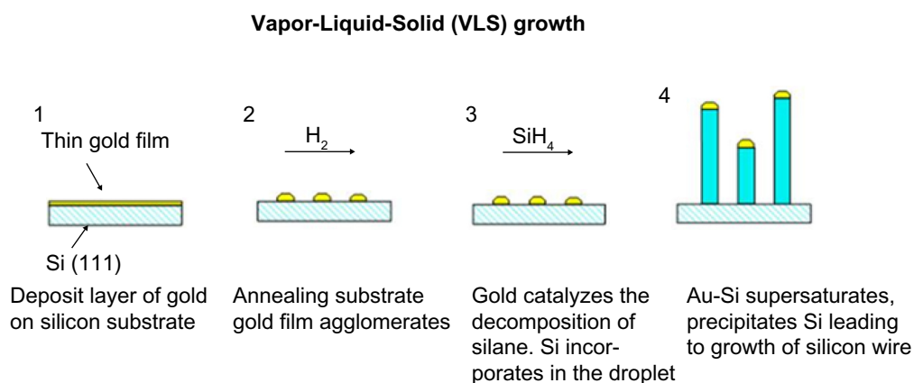
Figure 1. SiNW growth via the vapor–liquid–solid method with gold nanoparticles. (1) A thin layer of gold is deposited on silicon substrate. (2) The substrate is annealed to form individual gold nanoparticles. (3) Gold nanoparticles catalyze the decomposition of silane gas and incorporate Si into Au–Si eutectic droplets. (4) Supersaturated Si participated out of the droplets, forming anisotropic nanowires, having the same diameters as the gold nanoparticles.
