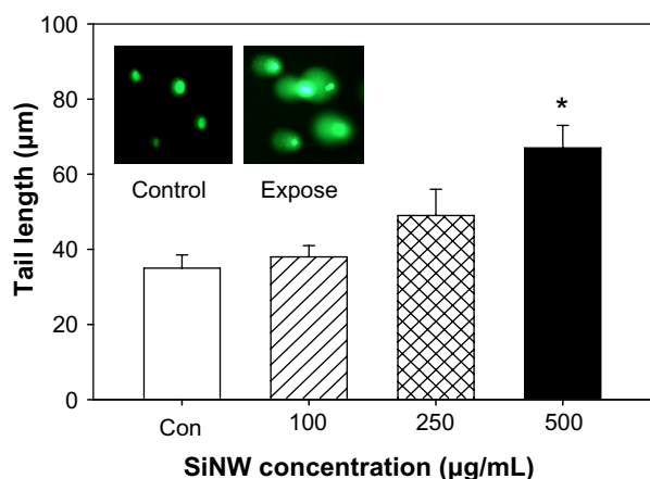
Figure 9. DNA damage in RAW 264.7 cells induced by SiNW as measured by the CometAssay. An increase in tail length represents increased DNA damage. Inset A shows control cells, inset B shows 500 µg/mL exposed cells. Data presented are means of \pm SEM for five sets of experiments at least 50 tail counts per experiment. *Significant increase in DNA damage compared to control cells ( P < 0.05 ).
