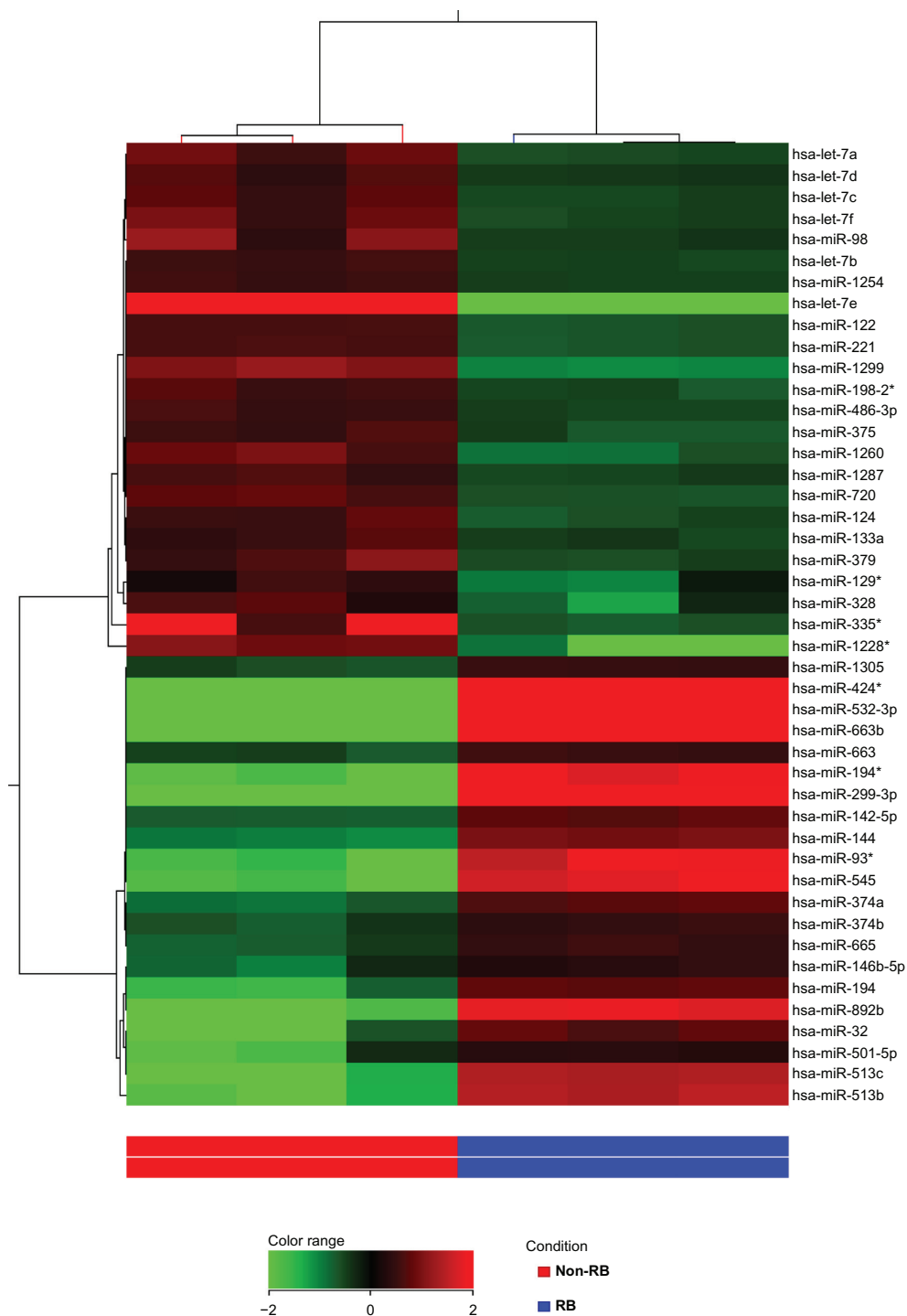
Figure 1. Hierarchical cluster shows differentially expressed miRNA between RB serum and age matched normal serum. Notes: The red colour indicates up-regulated miRNAs and the green colour indicates down-regulated miRNAs. The symbol (*) represents the miRNA minor.
