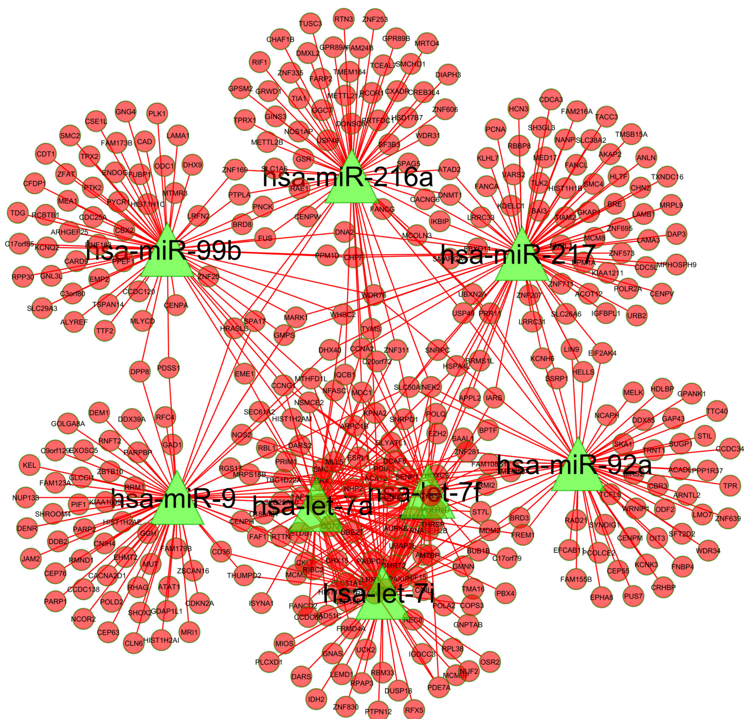
Notes: Green colored eclipses represent the miRNA and red colored eclipses indicate targeted genes for miRNA.
