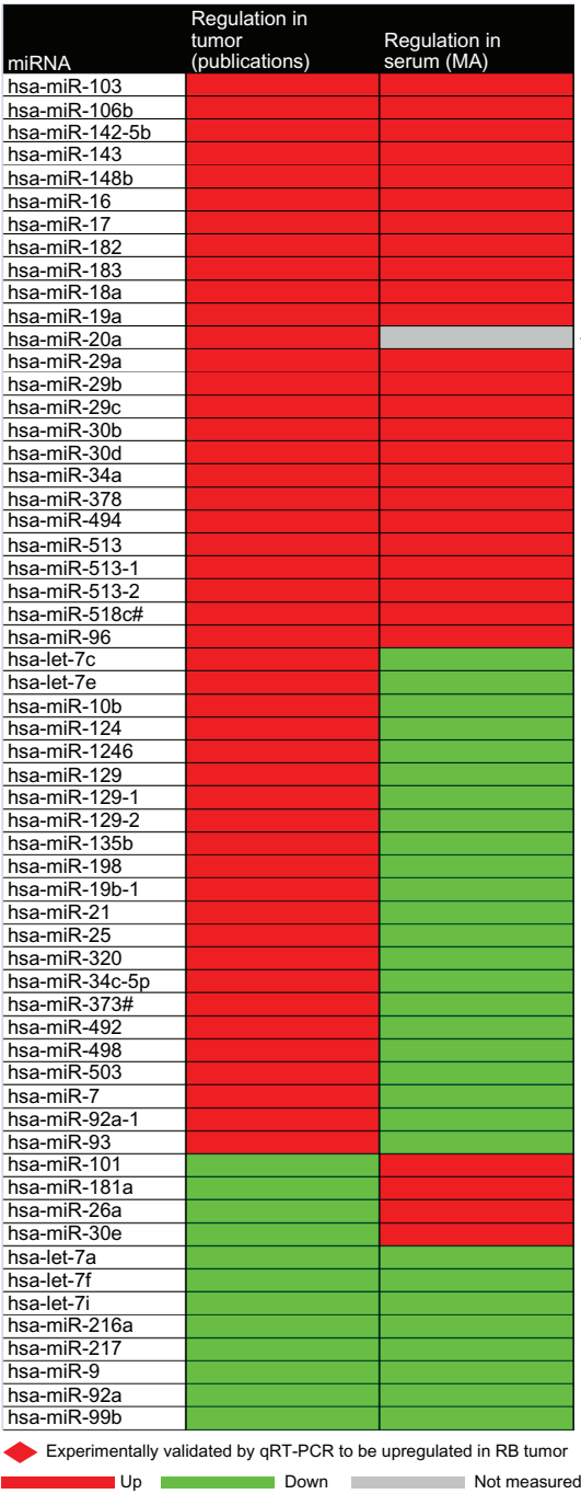
Figure 2. Hierarchical cluster shows common differential miRNAs in RB tumor and RB serum samples. Notes: The red color indicates upregulated miRNA, green color indicates downregulated miRNA, grey color indicates miRNA not measured in serum profile.
