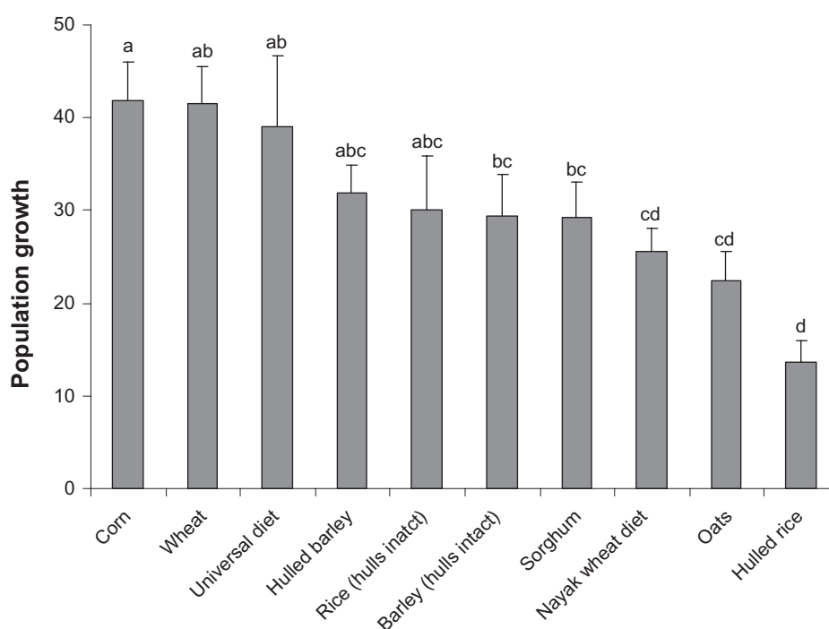
Figure 1. Mean ( \pm SE) population growth of Li. yunnaniensis on different diets. Note: Different letters on error bars mean significantly different populations using LSD test ( P < 0.001 ).
